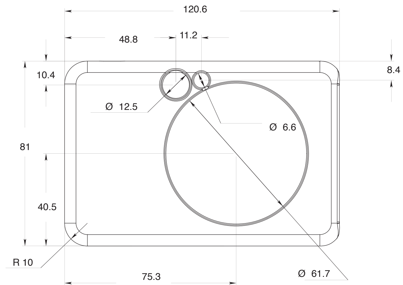
Front
