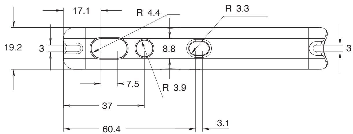
Front
